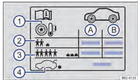
Fig. 193 Sticker with the tyre pressures.
