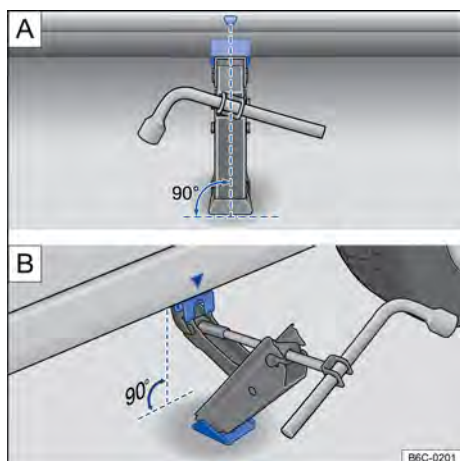
Fig. 202 Jacking points and vehicle jack at the rear left-hand side of the vehicle.
