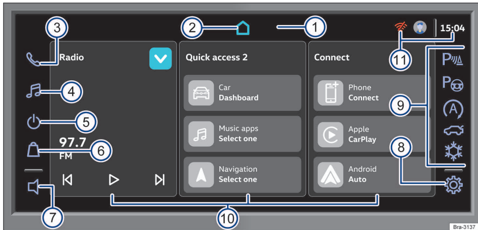
Fig. 138 Control overview.
