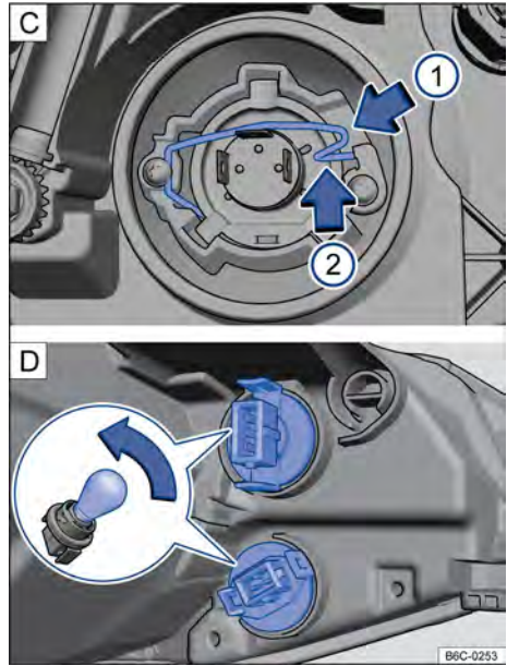
Fig. 167 In the engine compartment: high and low beam turn signal cover.
