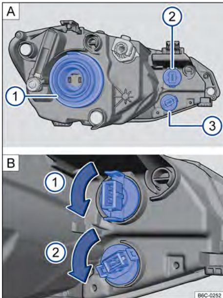
Fig. 166 In the engine compartment: headlight. ① Daytime running light and position light and ② Direction indicator.
