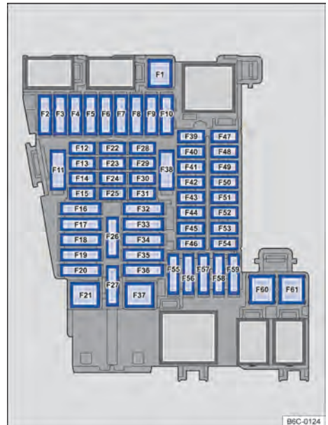
Fig. 173 On the dash panel: fuses arrangement.
