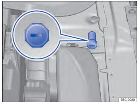
Fig. 179 On the engine compartment: jump starting point (grounding point).
