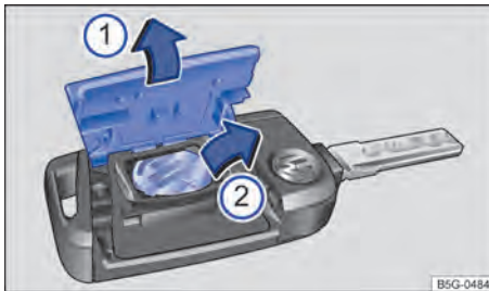
Fig. 53 Vehicle key: replacing the battery.
