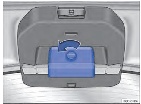
Fig. 50 On the rear lid: warning triangle holder.
