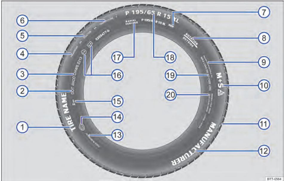
Fig. 197 International tyre lettering (example).
