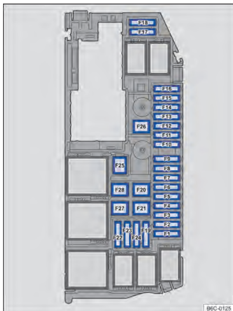
Fig. 175 In the engine compartment: fuse arrangement.
