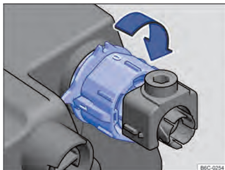
Fig. 74 In the engine compartment: headlight range adjustment switch.
