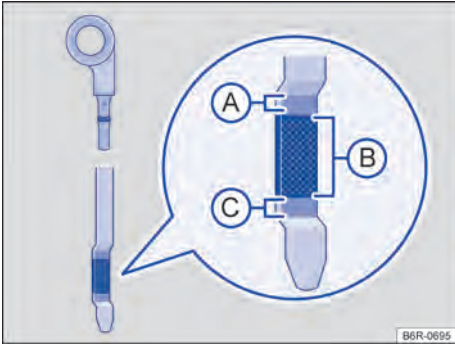
Fig. 185 Oil dipstick with markings.
