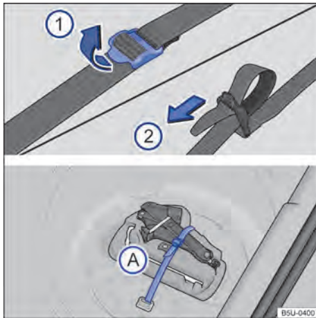
Fig. 160 On the luggage compartment: vehicle toolkit securing strap and vehicle toolkit.
